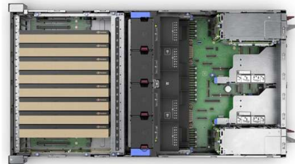
Figure 1. Top-down view of the HPE ProLiant Compute DL380a Gen12 showing eight double-wide GPUs
